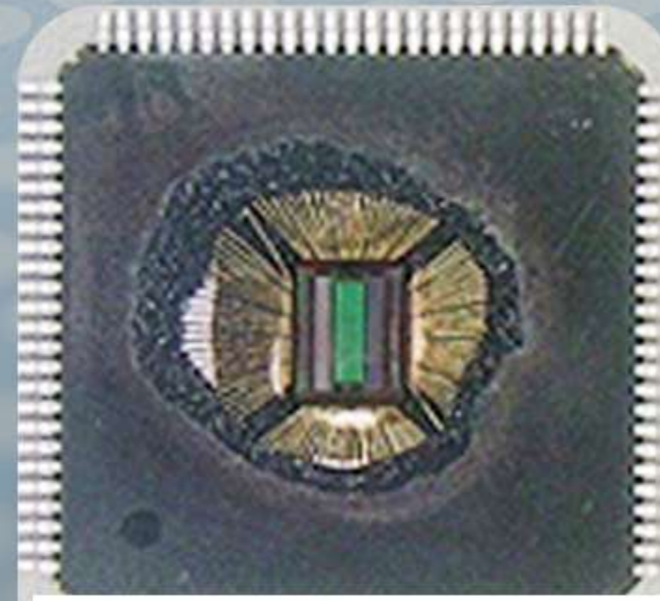
Decapsulation
